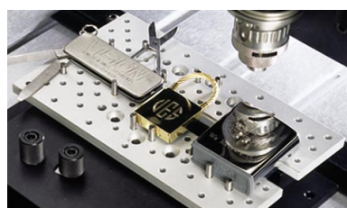
Tilbehør: Hul-jig, en universal holder for alle former for skilte.
